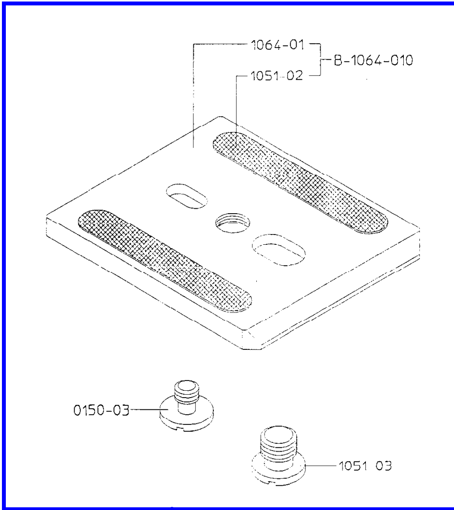
#1064 Wedge Plate, Complete
