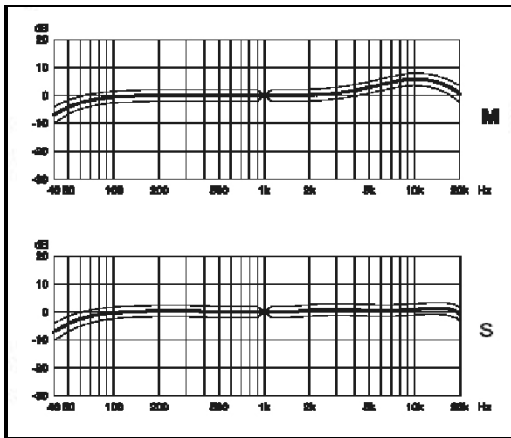
Frequency Response
