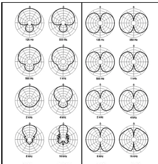
Polar Pattern M
