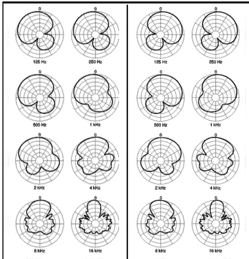
Polar Pattern L
